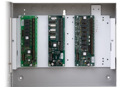
3 x I/O boards without PSU
